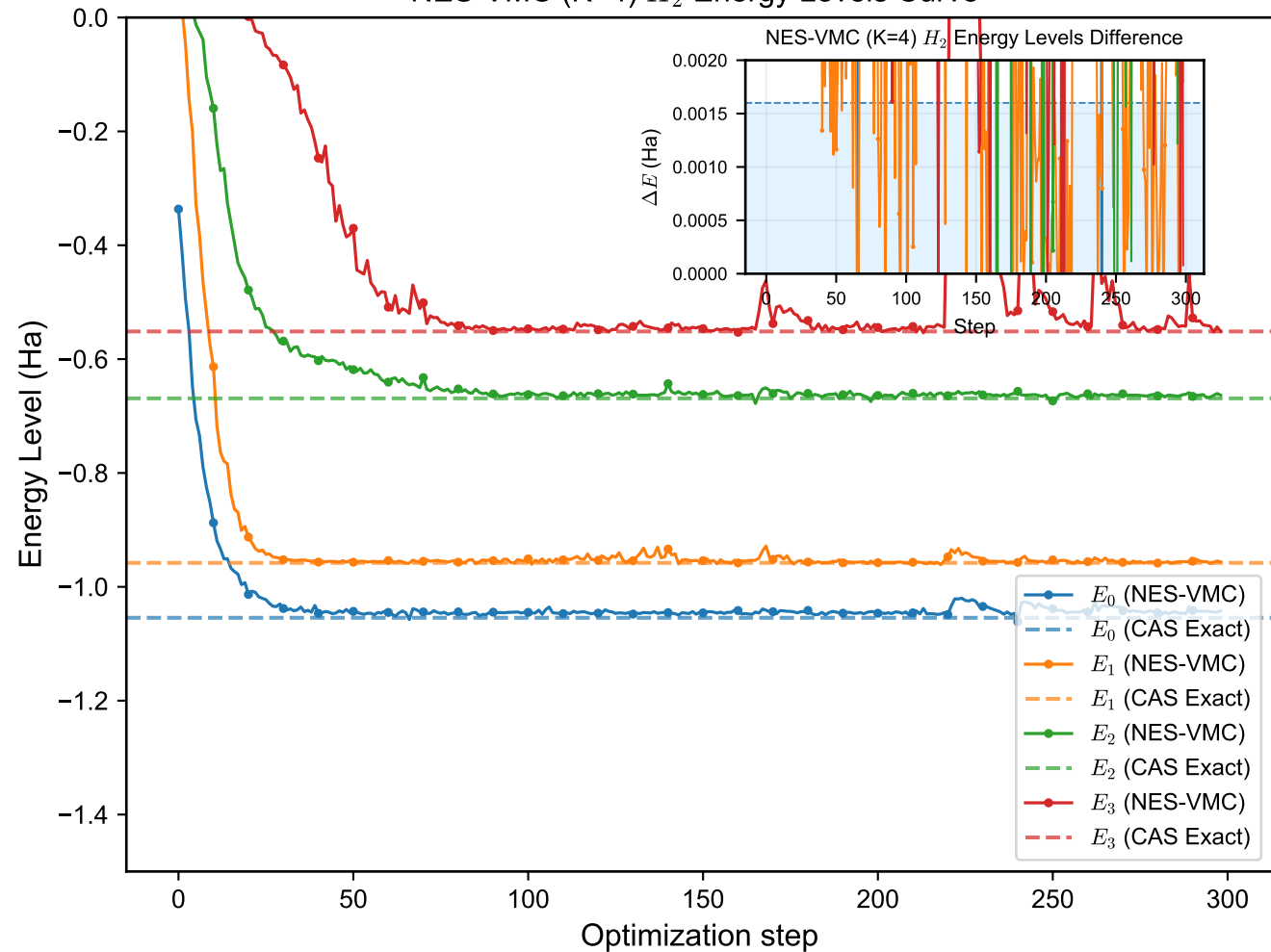
NES-VMC (K=4) H_2 Energy Levels Curve
